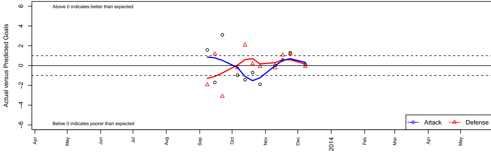
Vashon Riptide B97 Dots are actual minus expected GF (blue circles) and GA (red triangles). Blue line is smoothed change in attack strength. Red is smoothed change in defense strength.
